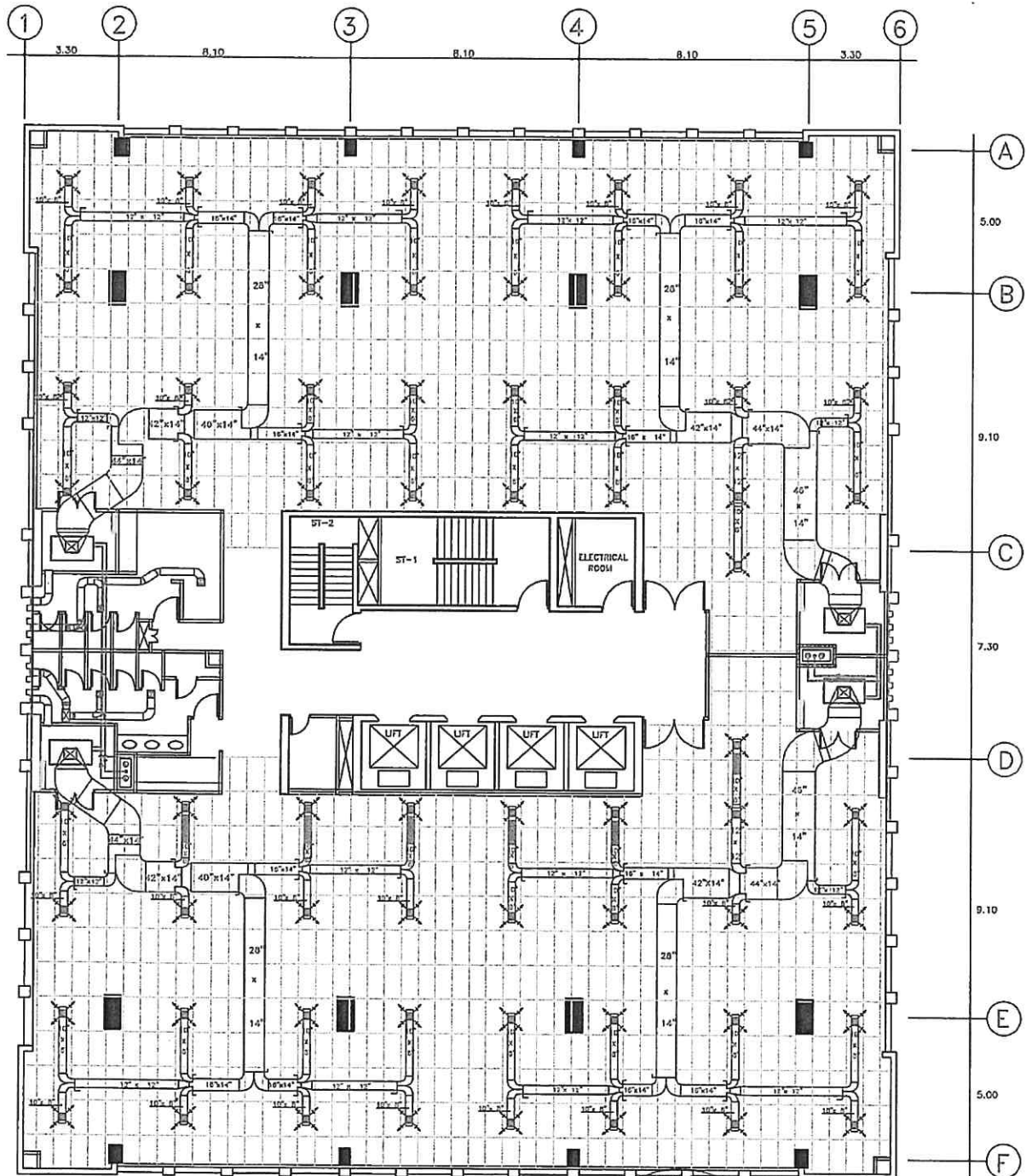
9th FLOOR PLAN AIR CONDITIONING SYSTEM
