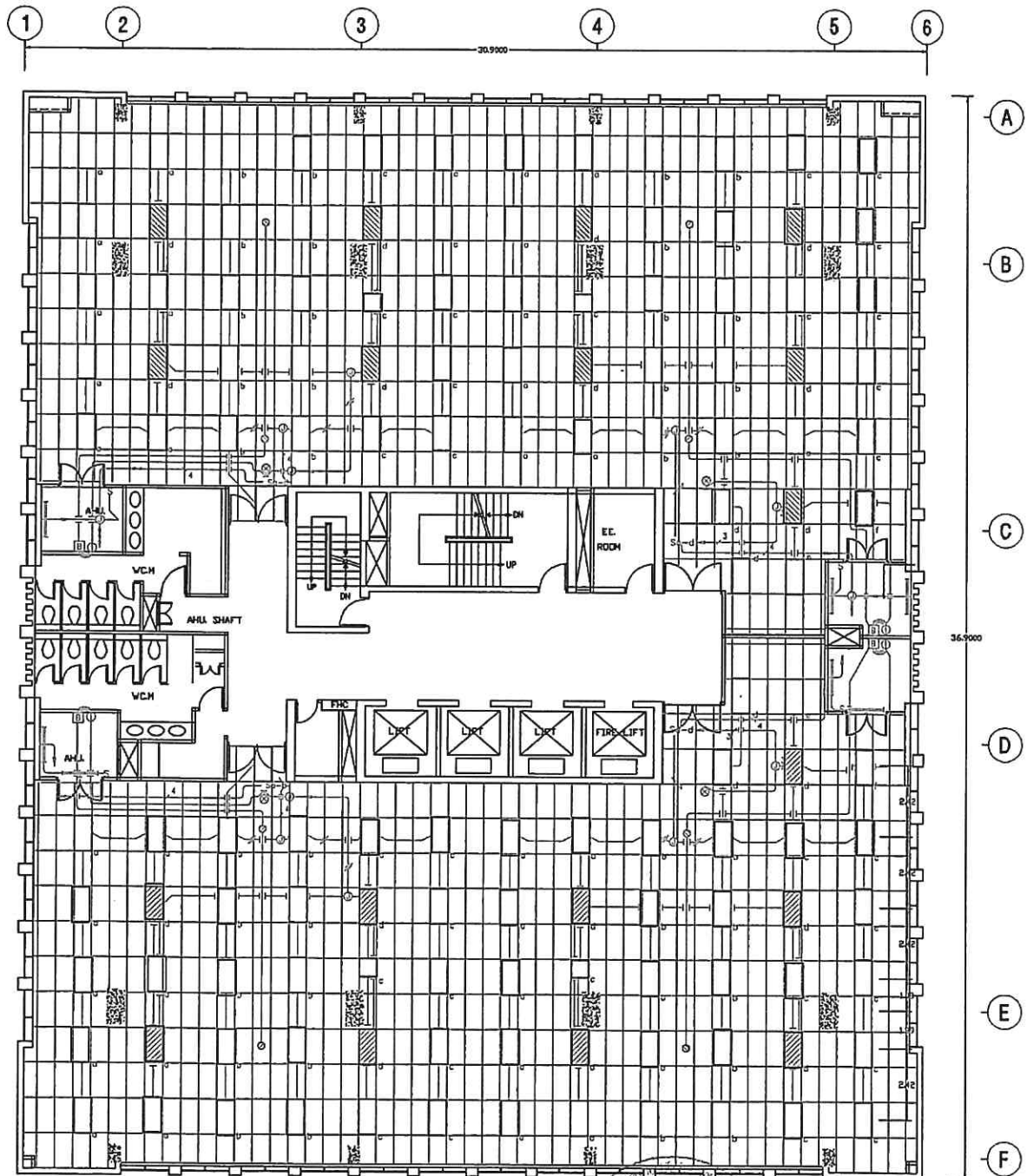
9th FLOOR LIGHTING PLAN
