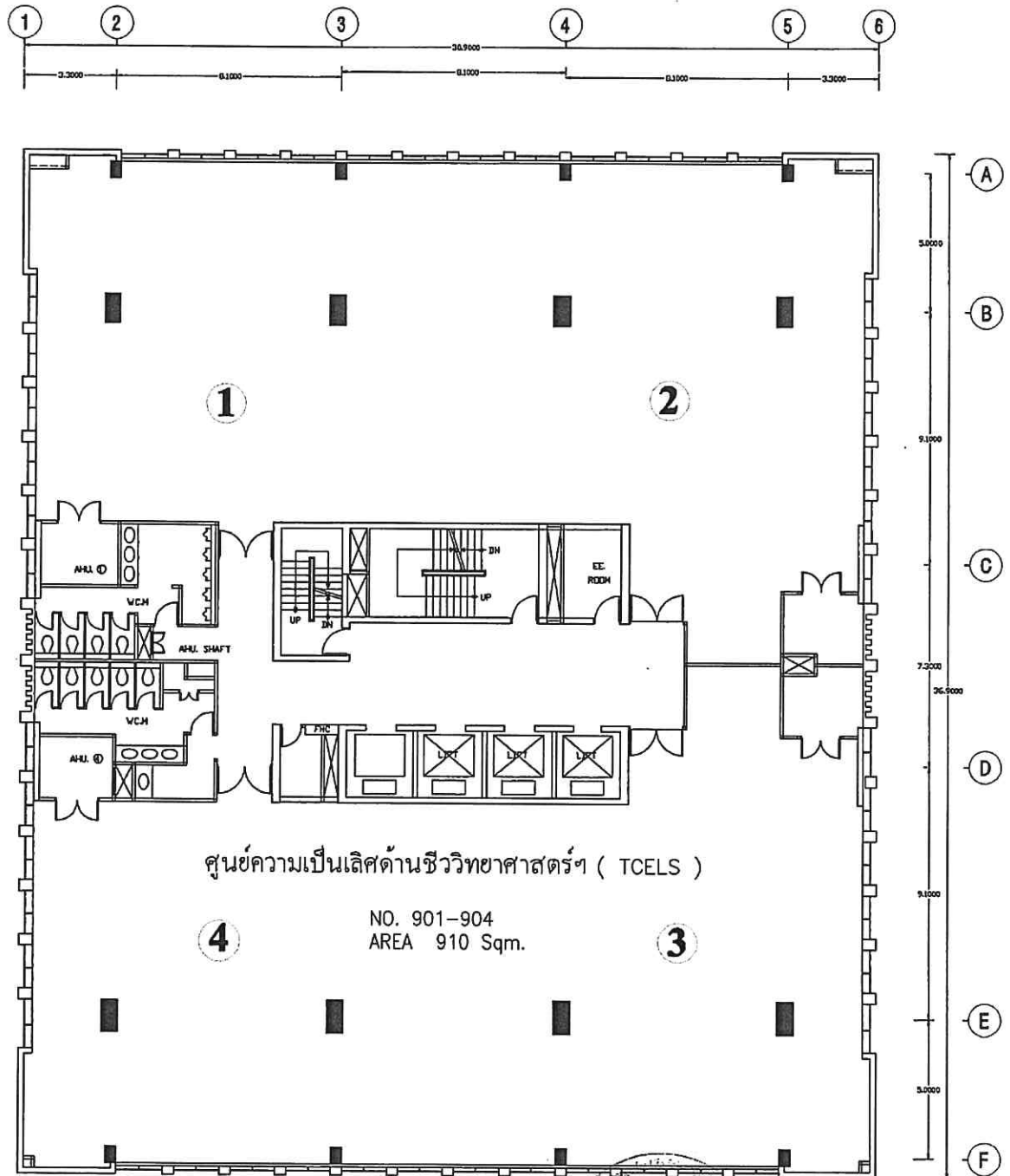
9th FLOOR PLAN
