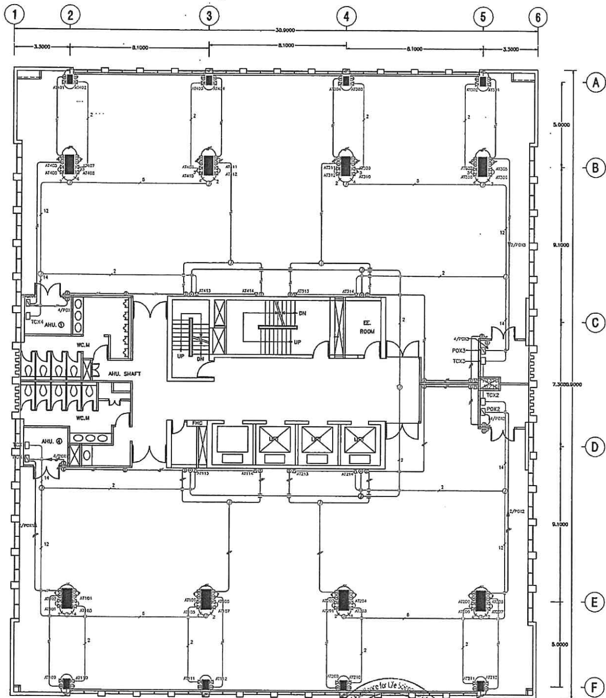
9th FLOOR RECEPTACLE, TELEPHONE & MATV OUTLET PLAN
