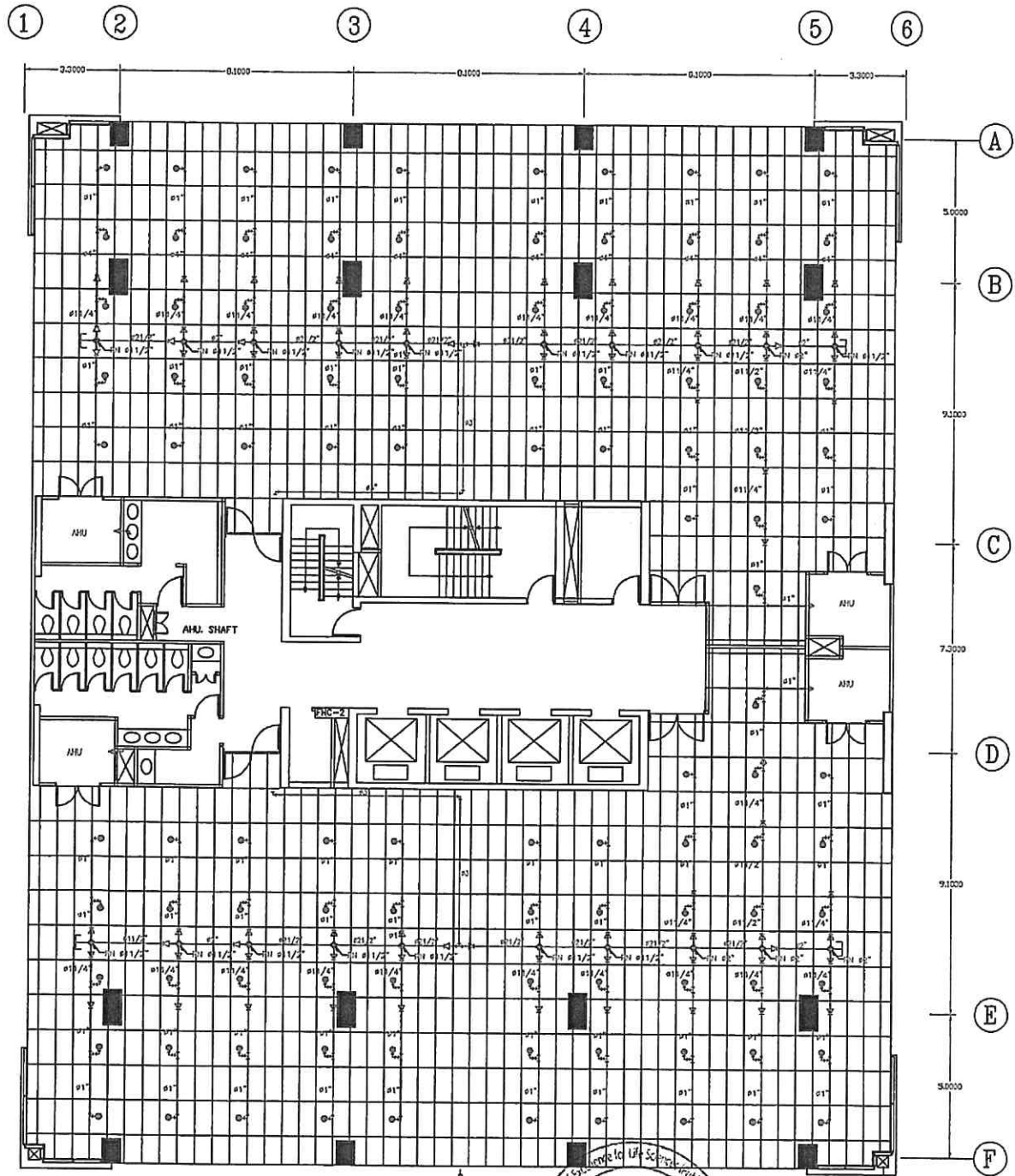
9th FIRE PROTECTION SYSTEM LAYOUT FLOOR PLAN
