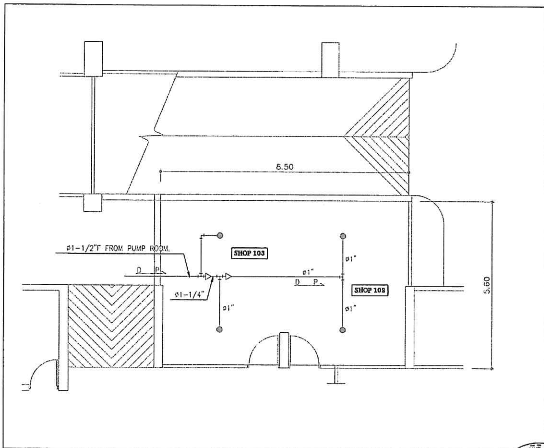
FIRE PROTECTION GROUND FLOOR PLAN
